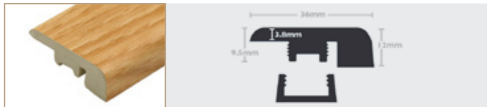
End Profile
