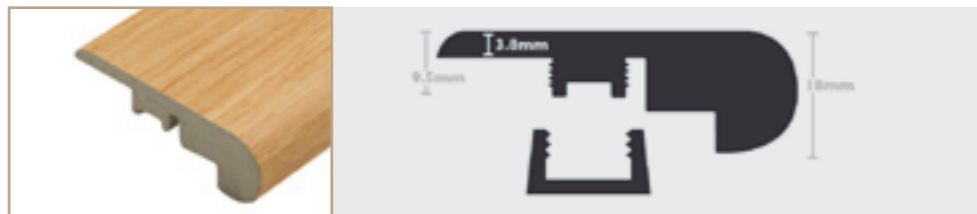
Stair Nosing
